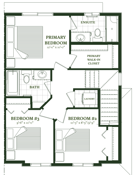
THIRD FLOOR
