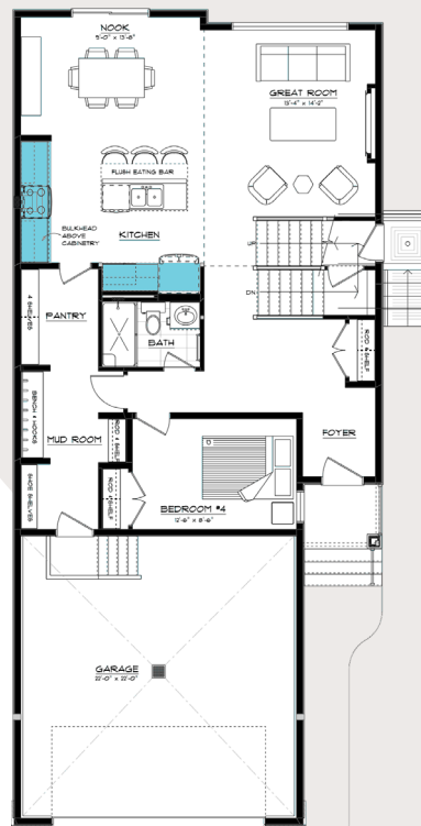
MAIN FLOOR
